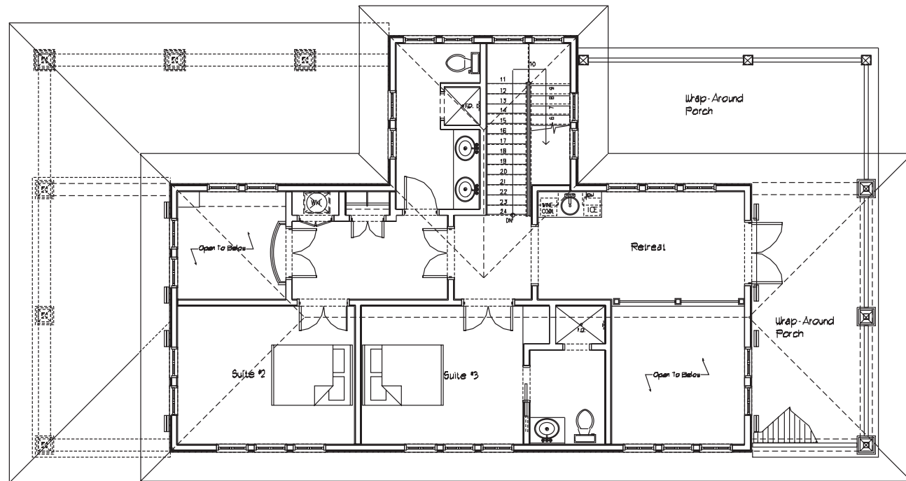
SECOND FLOOR
